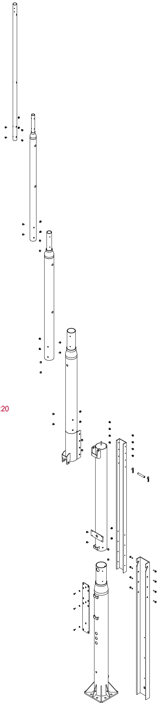
Esploso particolari palo / Exploded view mast's items
